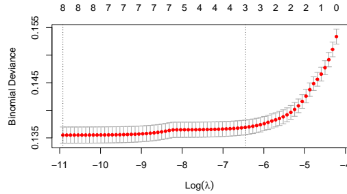
Figure 7: 10-fold Cross-Validation for Optimal \lambda in Lasso Regularization
